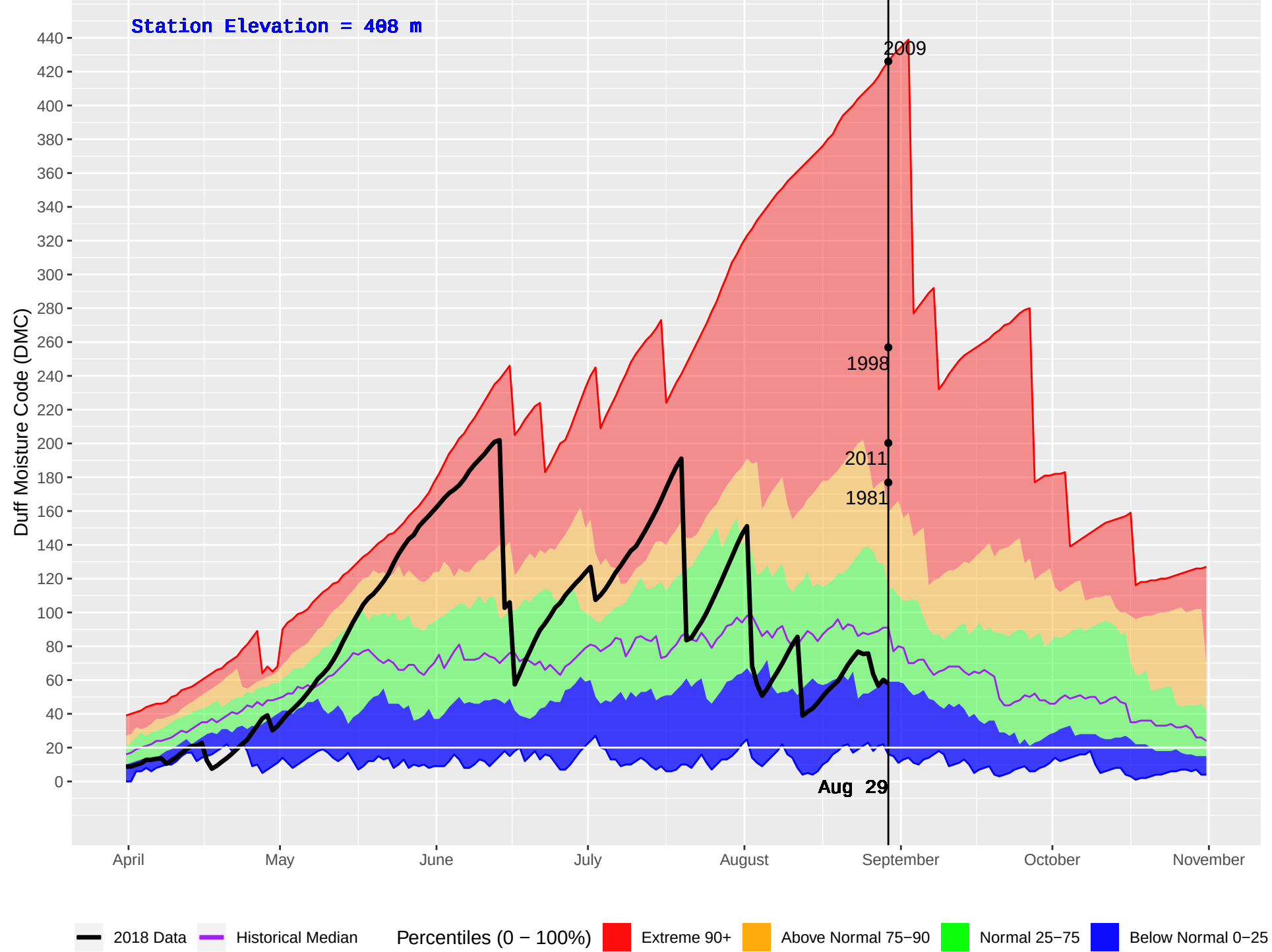
LILLOOET (280) : Historical (1977–2016) and Current (2018) Daily Duff Moisture Code (DMC)
