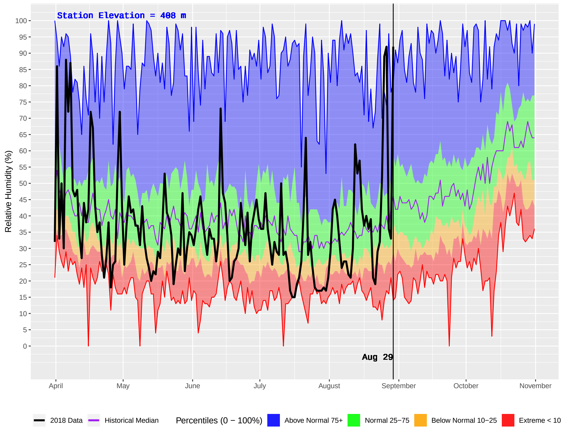
LILLOOET (280) : Historical (1977–2016) and Current (2018) Daily Relative Humidity
