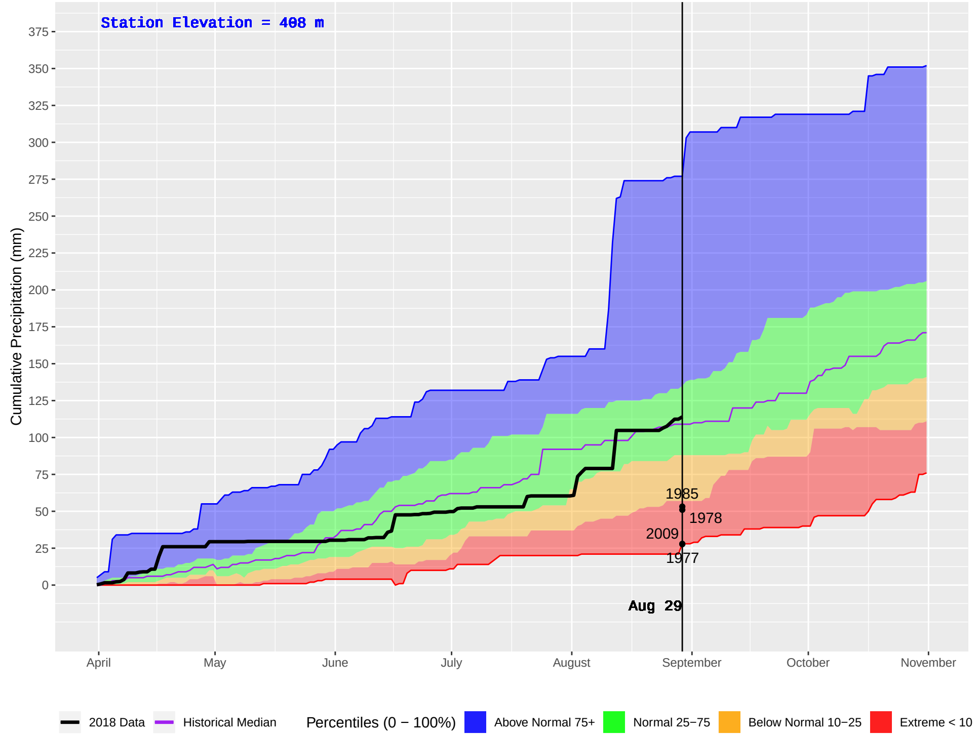
LILLOOET (280) : Historical (1977–2016) and Current (2018) Daily Cumulative Precipitation
