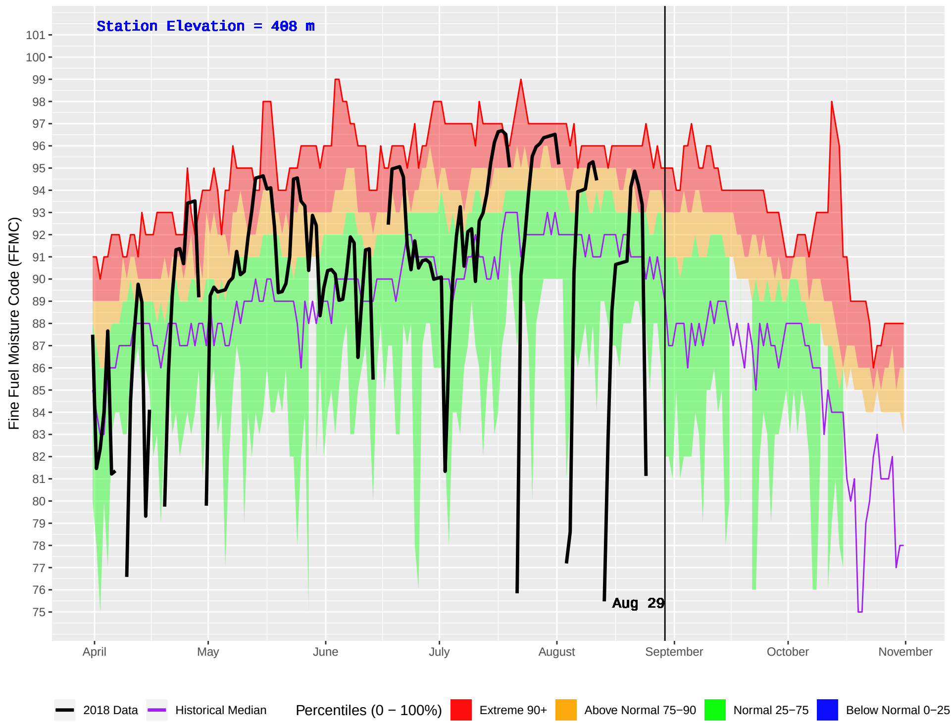
LILLOOET (280) : Historical (1977–2016) and Current (2018) Daily Fine Fuel Moisture Code (FFMC)
