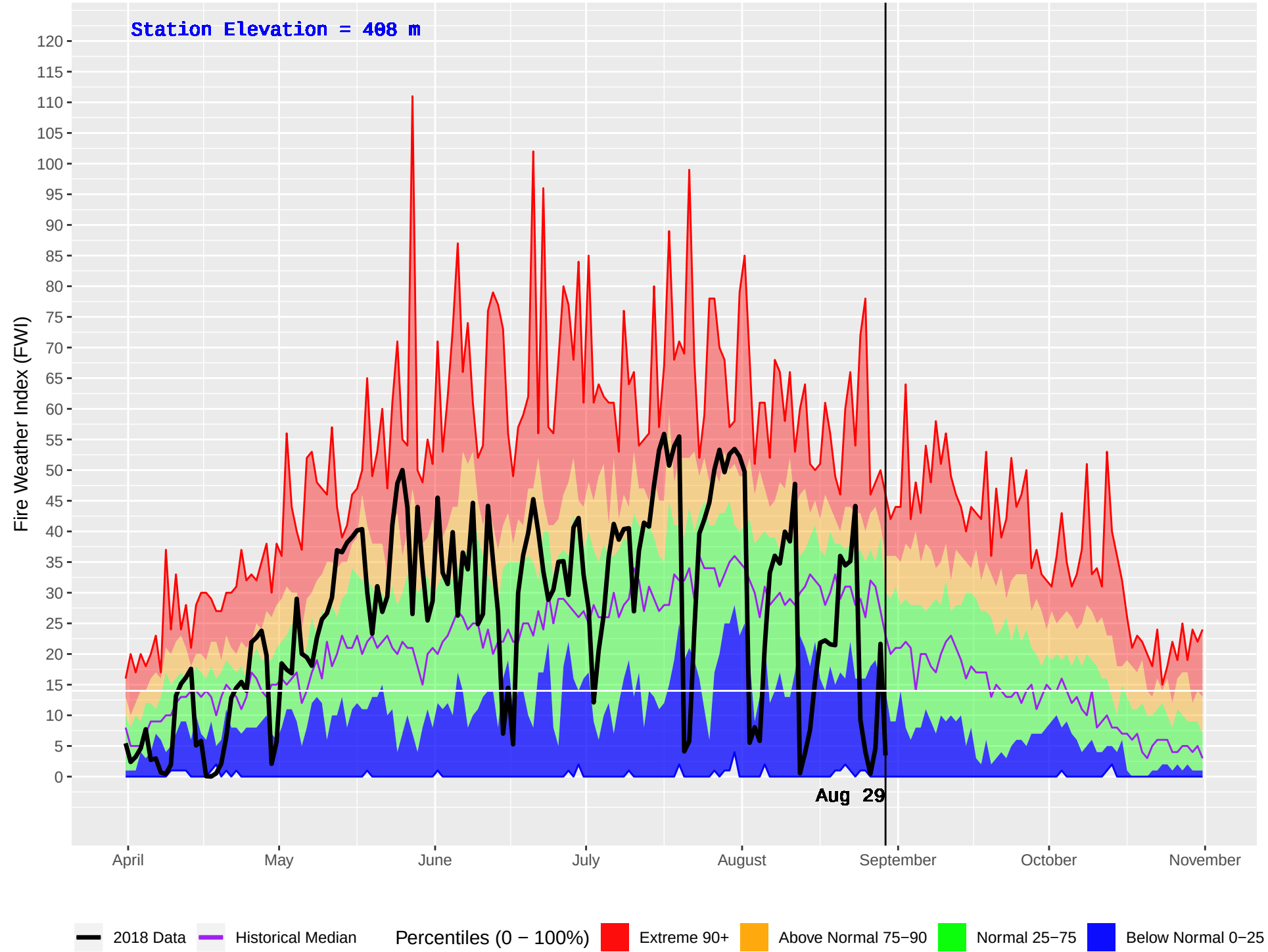
LILLOOET (280) : Historical (1977–2016) and Current (2018) Daily Fire Weather Index (FWI)
